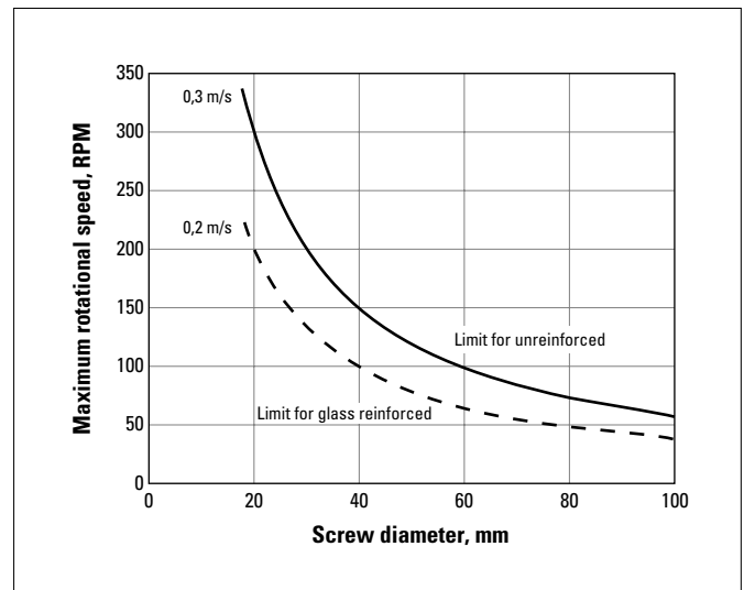
Fig. 3.6 Screw speed vs. screw diameter
