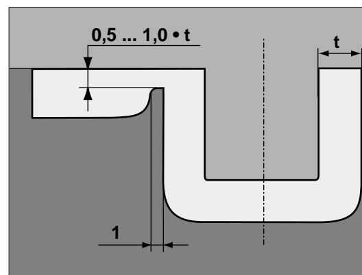
Fig. 4.8 Direct gate
