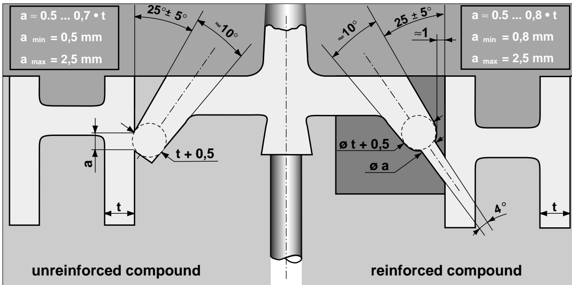
Fig. 4.6 Tunnel gates
